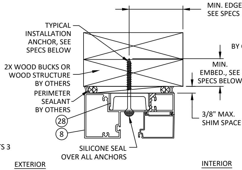
D 13 VERTICAL SECTION HEAD - WOOD FRAMING TYPICAL INSTALLATION
