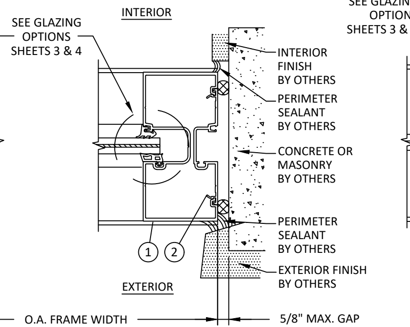
L HORIZONTAL SECTION 14 JAMB - DIRECT TO CONCRETE/MASONRY MEDIUM CONFIGURATION
