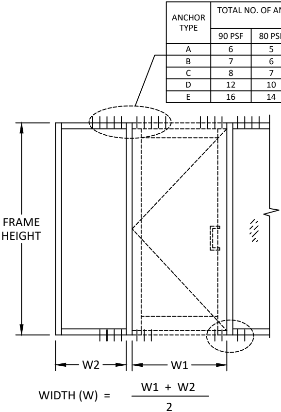
SINGLE DOOR
