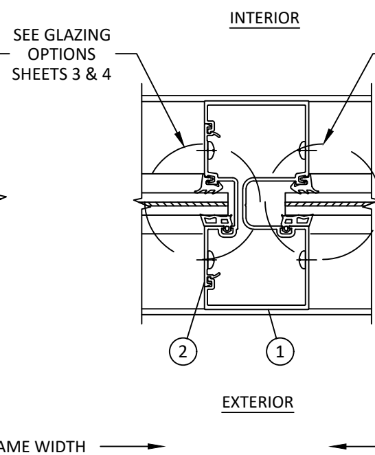
G HORIZONTAL SECTION 14 VERTICAL MULLION LIGHT CONFIGURATION
