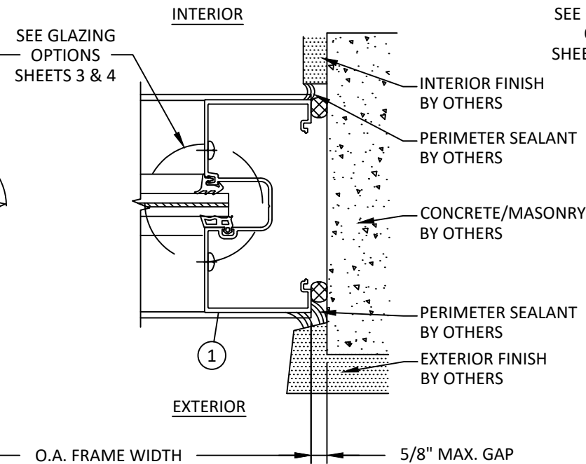
H HORIZONTAL SECTION 14 JAMB - DIRECT TO CONCRETE/MASONRY LIGHT CONFIGURATION
