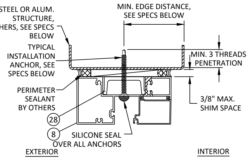
E 13 VERTICAL SECTION HEAD - METAL SUBSTRATE TYPICAL INSTALLATION
