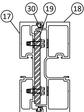
EXPANSION MULLION
